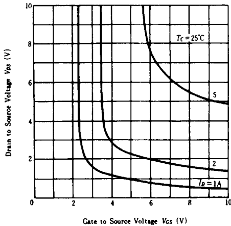
DRAIN - SOURCE VOLTAGE VS. GATE - SOURCE VOLTAGE
